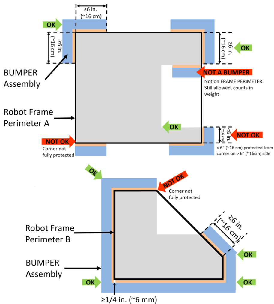
Figure 9-3 BUMPER corner examples
