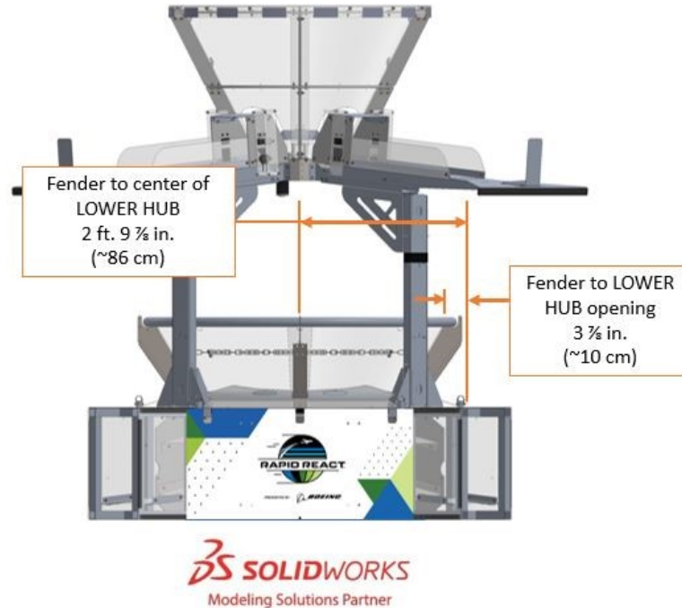
Figure 5-13 Fender geometry
