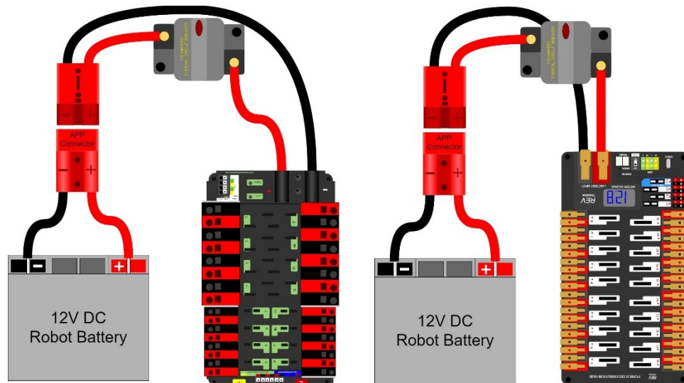
Figure 9-10 Electrical connection diagram
